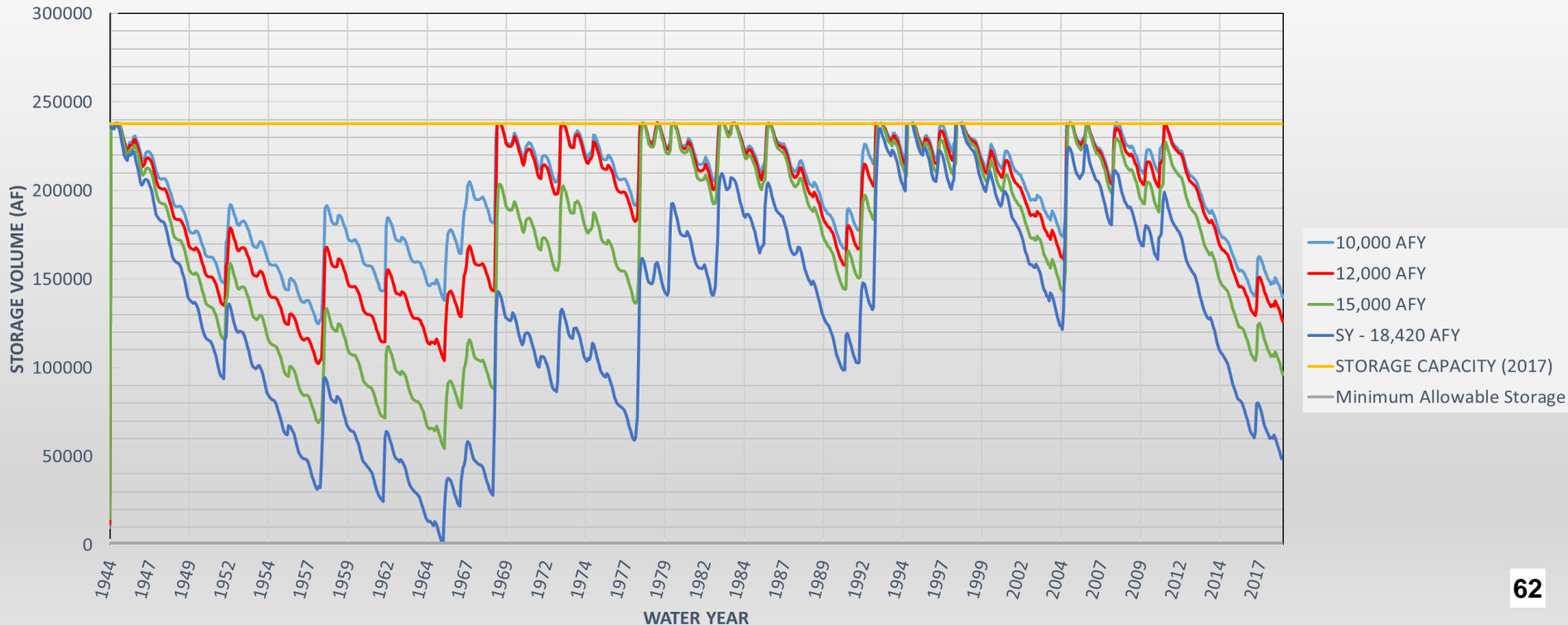
Lake Casitas Simulation with Constant Demands and Starting Reservoir Contents = 237,731 AF
