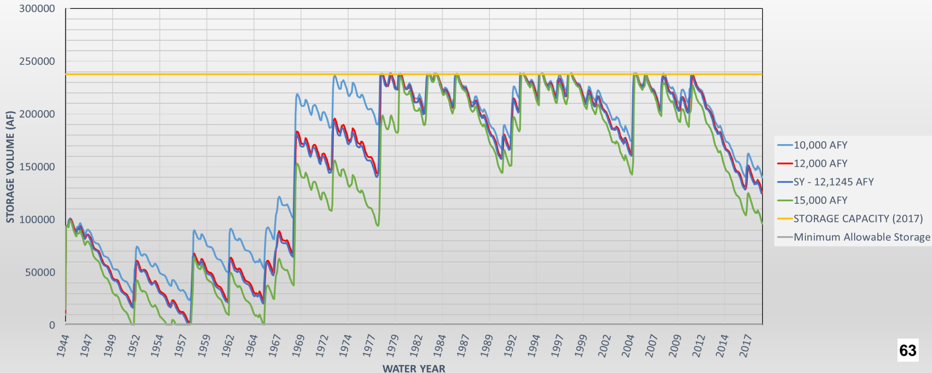
Lake Casitas Simulation with Constant Demands and Starting Reservoir Contents = 95,000 AF
